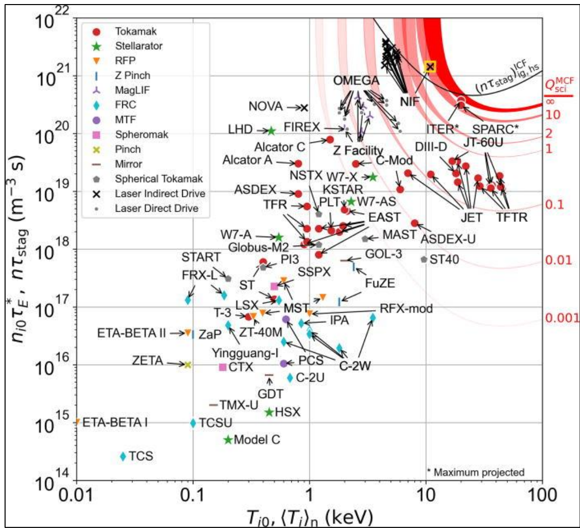
Figure 6: Progress Towards Fusion Energy Breakeven and Gain as Measured Against the Lawson Criterion 35 Colored contours are for scientific Q relevant to MCF (e.g., tokamaks). The black curve represents the hot-spot ignition condition for laser ICF.
