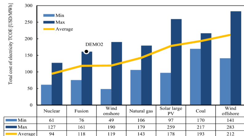
Figure 1: Total cost of electricity including external costs (TCOE). Source: Entler et al, 2018. 8
